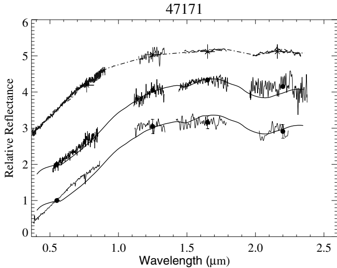
Fig. 3. Relative reflectance spectrum of (47171) 1999 TC 36 obtained in 2001 by Dotto et al. (2003) ( bottom ), in 2003 by Merlin et al. (2005) (shifted by 1 unit in reflectance) and in 2006 (this work) (shifted by 2.5 unit in reflectance). The two continuous solid lines represent the modeling suggested by Dotto et al. (2003), while in dashed-dot line is shown the best-fit modeling proposed in this work (see dashed-dot red line in Fig. 2).
