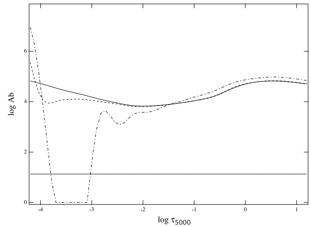
Figure 4. Equilibrium abundance stratification of cloudium [on the \log (N_X/N_H) + 12 scale] versus optical depth. Same legend as for Fig. 3 (the 100 G case is not shown). The horizontal grey line represents our initial standard homogeneous abundance (1.13) which is used as the starting value of the time-dependent simulations in this paper.
