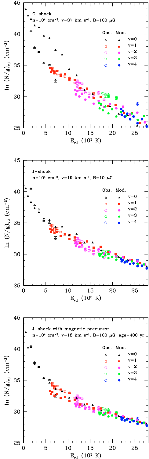
Fig. 6. H_2 Boltzmann diagrams of the B-zone compared with the predictions for a steady-state C-type and J-type shocks (top and middle panels) and for a J-type shock with a magnetic precursor (bottom panel). The shock model parameters are given in each panel and each vibrational state is labelled with a symbol, as indicated.
