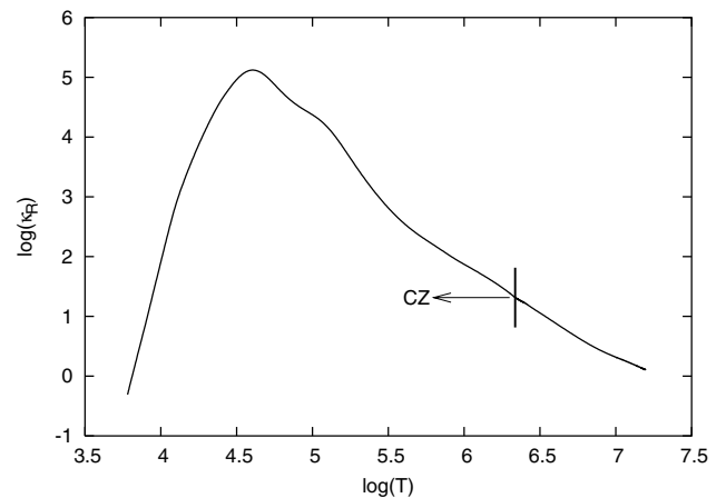
Figure 6. Rosseland-mean opacity from OPAL as used in the solar model BP04 of Bahcall & Pinsonneault (2004). The CZ is the region indicated with \log(T) \lesssim 6.34 .
