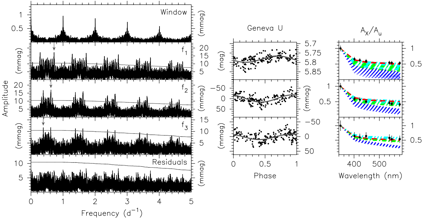
Fig. 6. Same as Fig. 2, but for f_1 = 0.72002(4) \text{ d}^{-1} , f_2 = 0.62125(5) \text{ d}^{-1} , and f_3 = 0.38271(8) \text{ d}^{-1} in the GENEVA U passband of HD 206540.
