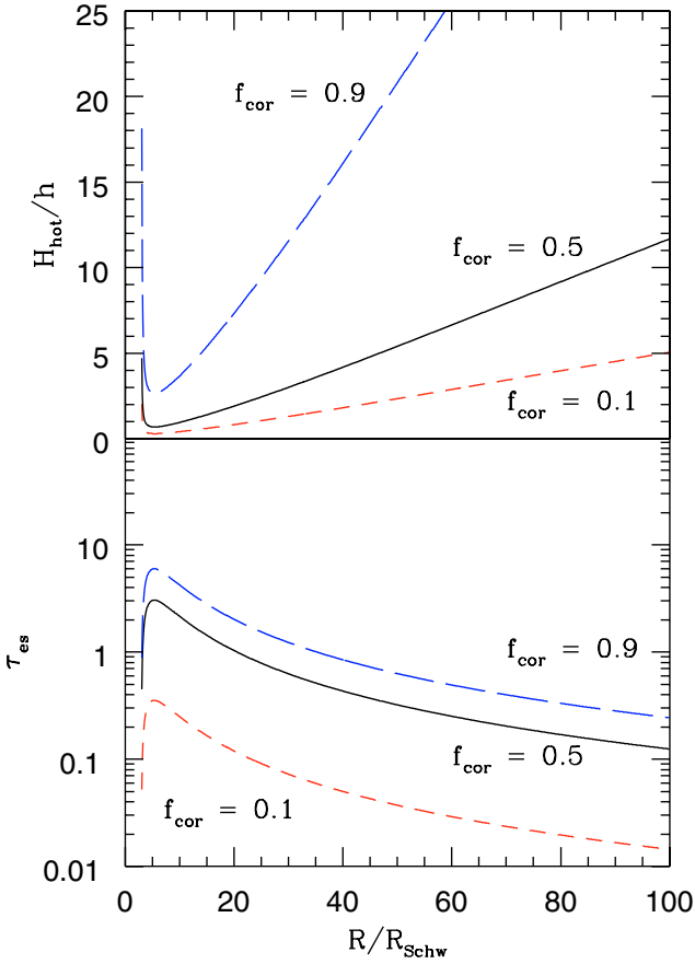
Fig. 3. Radial dependence of the thickness of the heated zone (in flare height units) and the optical depth of the heated zone directly at the flare position ( d = 0 ) for three values of the fraction of energy dissipated in the corona, f_{\text{cor}} . Other model parameters: M = 10^8 M_\odot , \dot{m} = 0.03 , f_{\text{cover}} = 0.1 .
