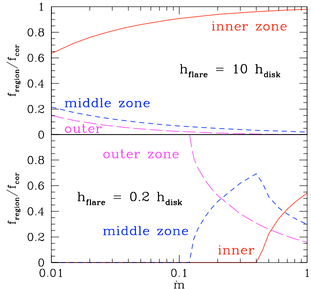
Fig. 9. The same as Fig. 8 but assuming that flares are located ten times higher above the disk ( upper panel ). Lower panel shows the solution appropriate for a magnetically heated disk skin ( f_{\text{cover}} = 1 , h_{\text{flare}} = 0.2h_{\text{disk}} ).
