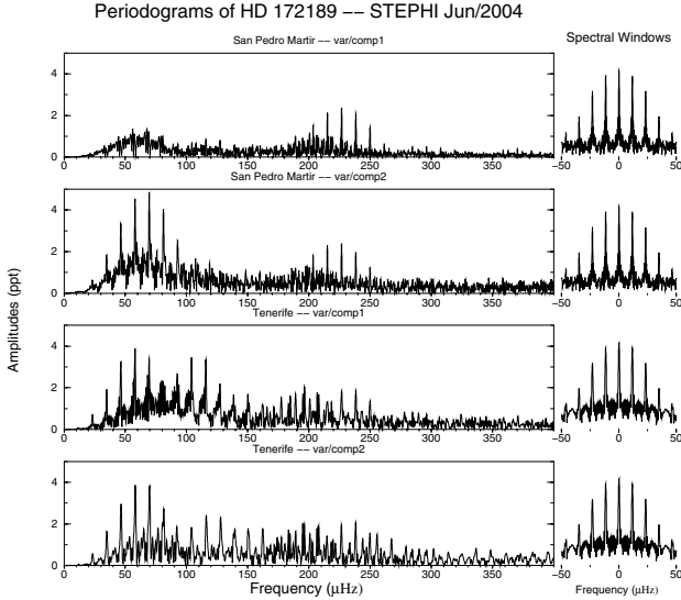
Fig. 2. Periodograms of the one-site light curves of var/comp1 and var/comp2 for the San Pedro Mártir and Tenerife data. In the right side are shown the respective one-site spectral windows.
