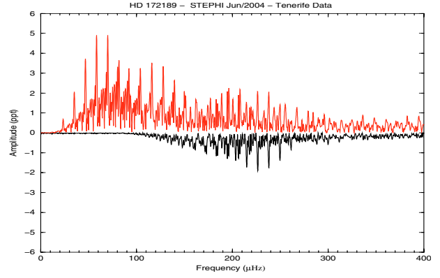
Fig. 3. Periodograms of the Tenerife data obtained with polynomial fitting of order 2 (top) and order 3 (bottom).
