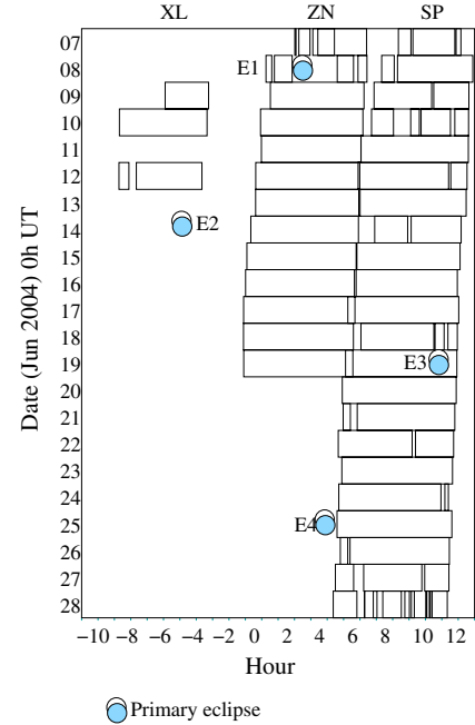
Fig. 1. Coverage diagram of the STEPHI XIII campaign. Each rectangular strip represents a night of observation. The labels XL, ZN and SP indicate the three observatories. The total number of hours of photometric data is 210 with an effective coverage of 40%. The times of minimum of the primary eclipses are indicated by E1, E2, E3 and E4.
