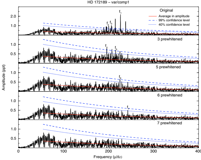
Fig. 5. Prewhitening process in HD 172189 (var/comp1). In each panel the peaks above the 99% confidence level (dashed line) are selected and removed from the original light curve, together with all previous selected frequencies, and a new periodogram is obtained. The selected peaks are indicated by f_1 , f_2 , etc. The lower level of 40% is indicated by the dotted curve and the solid curve represents the average amplitude.
