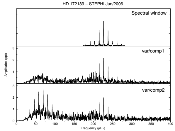
Fig. 4. Spectral window (top) and periodograms of the whole light curves of HD 172189 of var/comp1 (middle) and var/comp2 (bottom).
