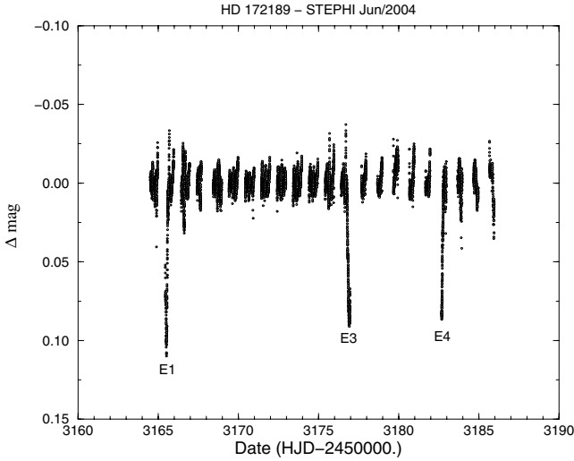
Fig. 6. Light curve of HD 172189. The measurements were binned to 60 s. Three primary eclipses, E1 , E3 and E4 are clearly visible.
