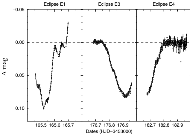
Fig. 7. The three primary eclipses ( E1 , E3 and E4 ) observed during the campaign. The points were binned and the pulsation frequencies were subtracted.
