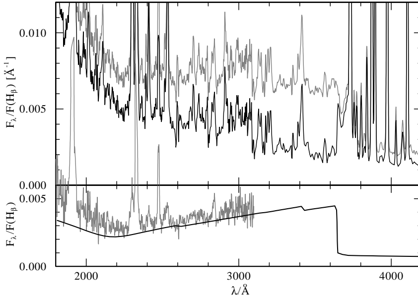
Fig. 2. Subtraction of the nebular continuum. Top panel: The observed flux distribution around the Balmer jump before and after subtraction of the nebular continuum. Bottom panel: The redened theoretical continuum as utilized for the nebular subtraction is plotted in black. It is compared to the nebular flux (grey) as estimated from the observation, by correcting for the stellar contribution (see text). Although the latter may still include a small contribution from the central star, the theoretical flux distribution is clearly confirmed.
