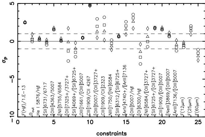
Fig. 7. Same as Fig. 6 but for models with different filling factors. Models defined by (n_0, \epsilon) equal to (1.05 \times 10^4 \text{ cm}^{-3}, 1.0) are represented by circles, (1.5 \times 10^4 \text{ cm}^{-3}, 0.49) by squares, (2.0 \times 10^4 \text{ cm}^{-3}, 0.27) by triangles, (3.0 \times 10^4 \text{ cm}^{-3}, 0.122) by diamonds.
