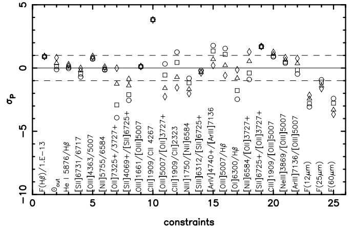
Fig. 9. The same as Fig. 8 for models ionized by a softened stellar flux (see text). Models defined by (n_0, \epsilon) equal to (7.5 \times 10^3 \text{ cm}^{-3}, 1.0) are represented by circles, (1 \times 10^4 \text{ cm}^{-3}, 0.6) by squares, (1.2 \times 10^4 \text{ cm}^{-3}, 0.4) by triangles, (1.4 \times 10^4 \text{ cm}^{-3}, 0.3) by diamonds.
