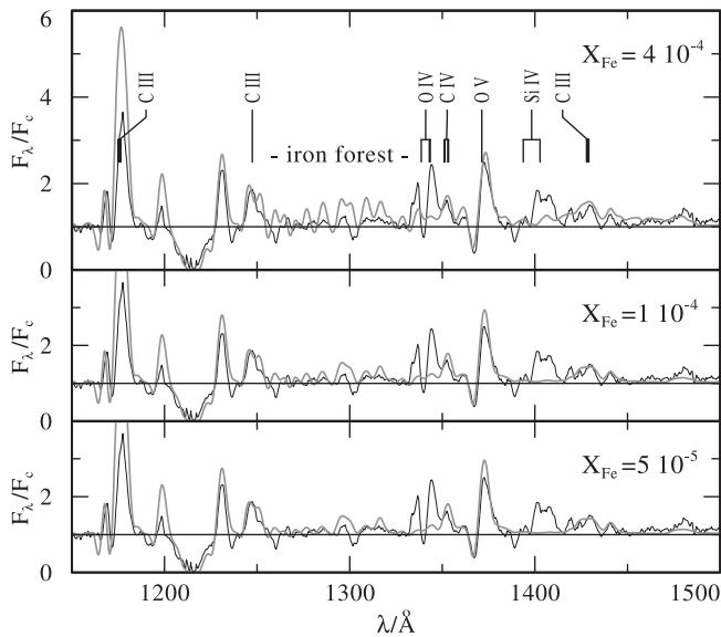
Fig. 4. Model calculations for different iron abundances. The strength of the iron forest indicates a significant iron deficiency on the central stars surface ( X_{\text{Fe}} < 1 \times 10^{-4} ).
