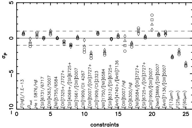
Fig. 10. Models ionized by a softened stellar flux (as in Fig. 9), with an inner density n_0 = 1.4 \times 10^4 \text{ cm}^{-3} and a nebular filling factor \epsilon = 0.3 (the best combination of Fig. 9). Now, the inner 3 \times 10^{-3} M_\odot of the nebula are He- and C-rich. The abundances of He and C (by number relative to H) are: 1.04 and 0.4 (circles), 0.78 and 0.3 (squares), 0.52 and 0.2 (triangles), 0.26 and 0.1 (diamonds). Otherwise, the abundance ratios with respect to hydrogen are (by number): H: He: C: N: O: Ne: S: Ar = 1: .09: 4.0 \times 10^{-4} : 3.95 \times 10^{-5} : 2.65 \times 10^{-4} : 4.26 \times 10^{-5} : 4.0 \times 10^{-6} : 8 \times 10^{-7} .
