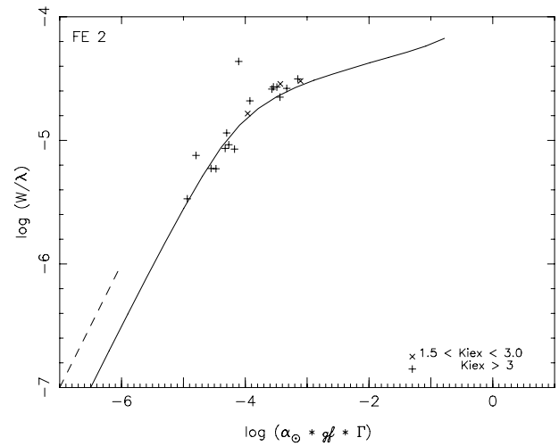
Fig. 4. Observed curve of growth for Fe II in TW CMa. The full line represents the theoretical curve of growth for a typical line ( \lambda = 5000 \text{ \AA} , \chi_{\text{ex}} = 3 ). The atmospheric parameters adopted for this star are T_{\text{eff}} = 5364 \text{ K} , \log g = 1.0 , v_t = 4.0 \text{ km s}^{-1} , and [\text{Fe}/\text{H}] = -0.5 \text{ dex} . The dashed line on the left shows the [\text{Fe}/\text{H}] = 0 location.
