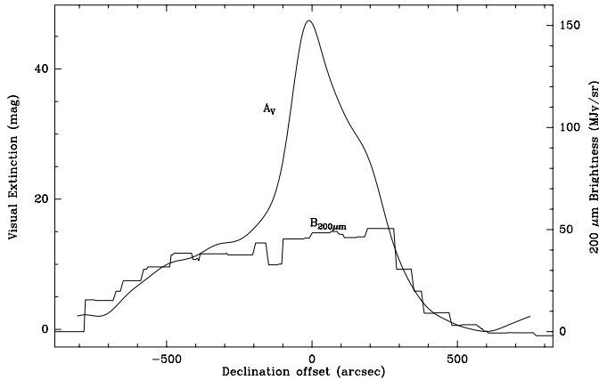
Fig. 6. ISOPHOT 200 \mu\text{m} cold dust emission and visual extinction (smoothed to 90'' ) cuts through Peak 1 (cut location is shown in Fig. 5). The dust peak is not visible at all in the 200 \mu\text{m} emission. Left is south, right is north.
