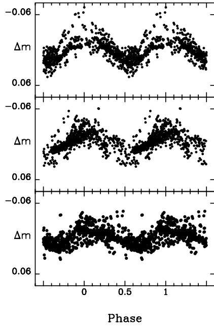
Fig. 7. Phase diagrams for f_1 = 2.1066 \text{ cd}^{-1} (top), f_2 = 1.8694 \text{ cd}^{-1} (middle) and f_3 = 2.2124 \text{ cd}^{-1} (bottom). In each panel, the data have been prewhitened to remove the other two frequencies.
