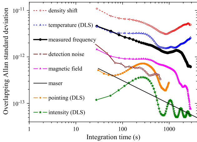
FIG. 4 (color online). Stability analysis based on the overlapping Allan standard deviation. The frequency measurement (solid black dots) yields a stability of 4.6 \times 10^{-12} at one shot, corresponding to 2.4 \times 10^{-11} at 1 s. All relevant noise sources are measured independently (see text) and are shown here as frequency noise. The periodic modulation in some of the curves reflects the air-conditioning cycle of 10 min.
