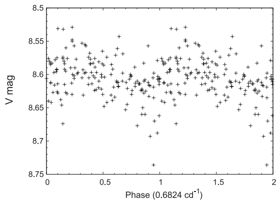
Fig. A.18. Phase plot of HD 173292 folded with the frequency 0.6824 \text{ c d}^{-1} for the ASAS-3 dataset.
