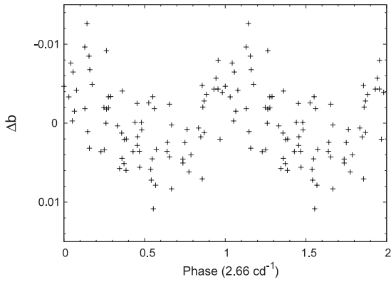
Fig. A.13. Phase plot of HD 51193 folded with the frequency 2.66 \text{ c d}^{-1} in the b filter for the OSN data obtained in 2004.
