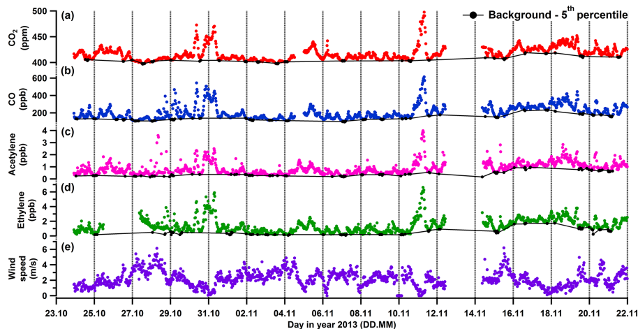
Figure 1. (a–d) Temporal variation of the mole fraction of selected compounds monitored during the Multi- \text{CO}_2 campaign (30 min time step). The black lines represent the background levels defined with the calculation of the 5th percentile (black disks). (e) Wind speed during the campaign. Time is given in UTC.
