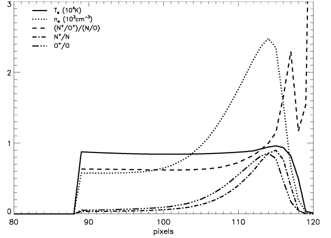
Figure 4. Variation of some local properties in the 3D grid of the model, along the large axis of the nebula (i.e. crossing the knots). Solid line: T_e ( 10^4 K); dotted line: n_e ( 10^3 \text{ cm}^{-3} ); dashed line: (N^+/O^+)/ (N/O) ; dash-dotted line: N^+/N ; and dot-dot-dashed line: O^+/O . Note that in this figure the pixels range from 80 to 120.
