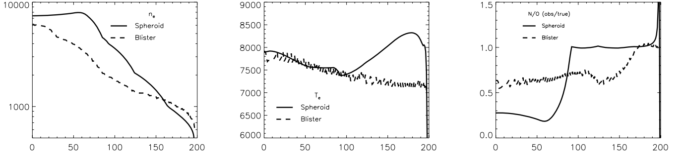
Figure 17. Variation of some ‘apparent’ parameters (from left to right: n_e , T_e and N/O ), determined from the emission-line ratios shown in Fig. 15. Solid line: spherical model; dashed line: blister model.
