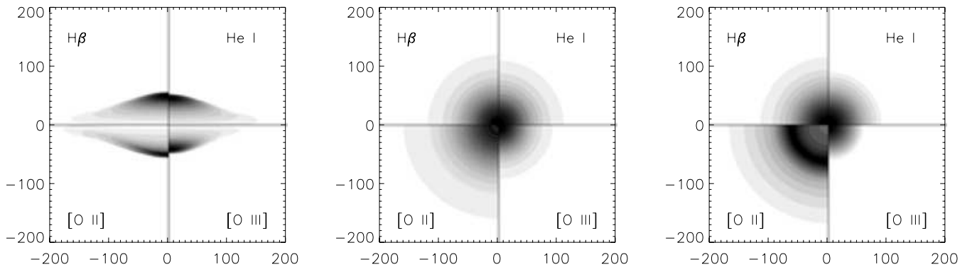
Figure 14. Synthetic H\beta , \text{He I } 6678 \text{ \AA} , [\text{O II}] 3726, 3729 \text{ \AA} and [\text{O III}] 5007 \text{ \AA} surface brightness maps (from upper left to lower right in each panel). Left panel: the blister model seen tangentially (in this case the maps for [\text{O II}] 3726, 3729 \text{ \AA} and [\text{O III}] 5007 \text{ \AA} are upside down); central panel: the blister model seen face-on; right panel: the spherical impostor model.
