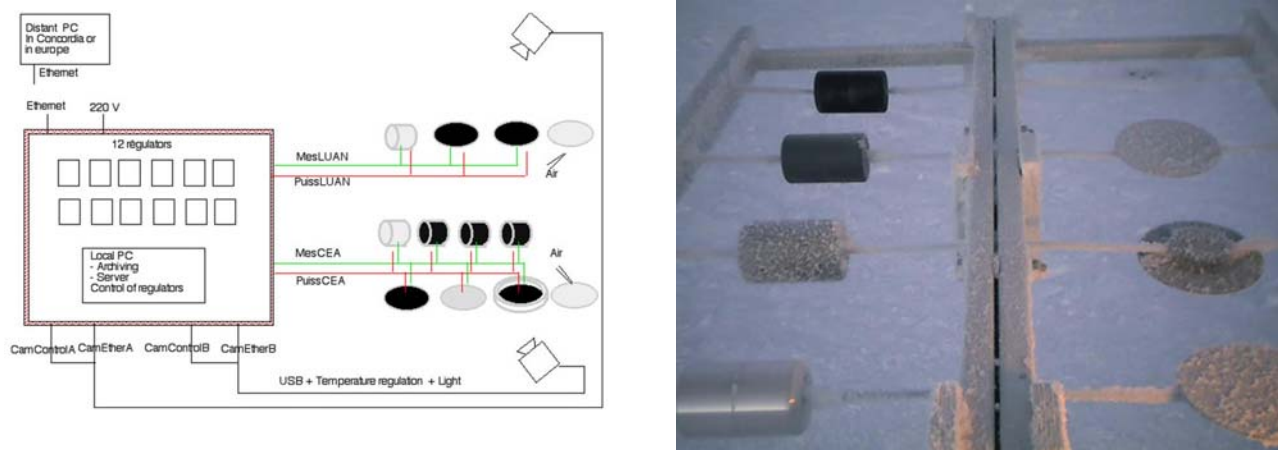
Fig. 8 The icing experiment GIVRE. Left : Schematic set up and read-out scheme. The test cells are a series of black and shiny cylinders and disks. These are observed during night with two webcams. Right : Typical icing one day after cleaning. Cylinders (from bottom to top): shiny aluminium cylinder; black cylinder without heating; black cylinder kept at air temperature; black cylinder kept 5^{\circ}\text{C} above ambient. Disks without heating and one side black, other side aluminium (from bottom to top): aluminium-side facing sky; black-paint side facing sky; again aluminium facing sky; and disk with teflon both sides.
