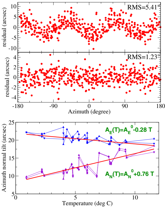
Fig. 9 Top: Residuals of the STELLA altitude model in arc seconds as a function of azimuth A in degrees. The top panel shows the residuals of a pure classic model with a clear 3A wave, while the lower panel shows the fit after including three empirical terms (see text). Bottom: Dependence of the azimuth axis alignment parameters A_N and A_E on the ambient temperature T along with the corresponding fits. Shown is again the case of the STELLA-II telescope. The effect is below 1'' per ^{\circ}\text{C} .
