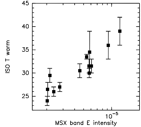
Fig. 7. Temperature (K) of the warm grey body needed to fit the dust spectra versus the MSX band E (18.2–25.1 \mu\text{m} ) intensity toward the sources presented in this paper.
