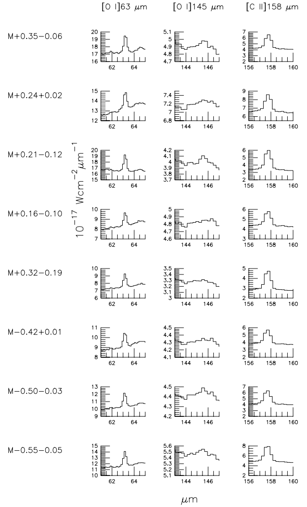
Fig. 4. Sample of LWS01 spectra of selected lines.
