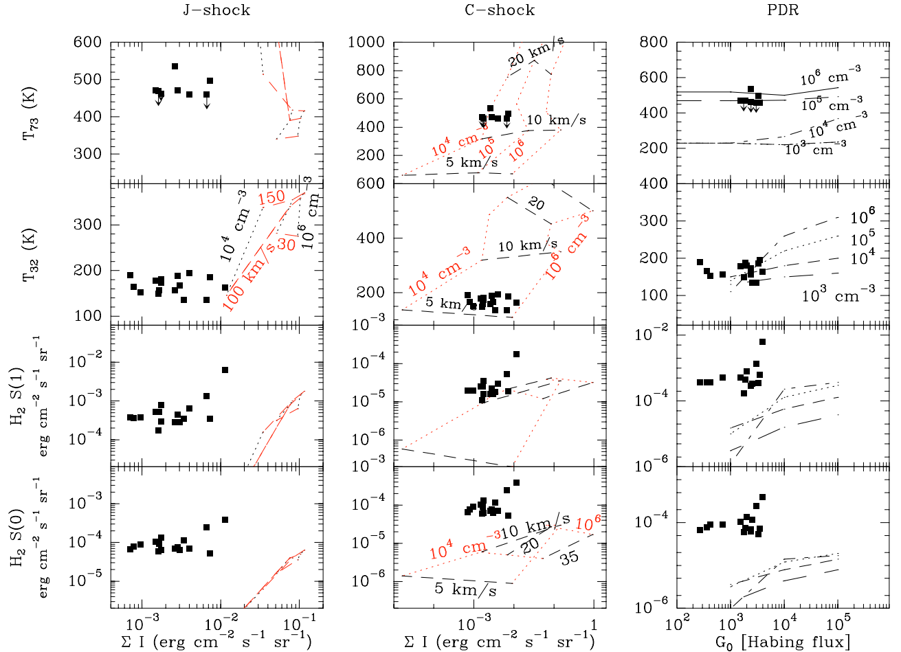
Fig. 11. Left panel: \text{H}_2\text{S}(0) and \text{H}_2\text{S}(1) intensities and rotational temperatures derived from the J = 3 and J = 2 levels ( T_{32} ) and from the J = 3 and J = 7 levels ( T_{73} ). All those parameters are plotted versus the total intensity radiated by lines. For comparison, the expected results for J-shocks models with different densities (dotted lines) and velocities (dashed lines) are also shown. Middle panel: same for C-shocks. Right panel: \text{H}_2\text{S}(0) , \text{H}_2\text{S}(1) , T_{32} and T_{73} versus G_0 and comparison with PDR models with different densities.
