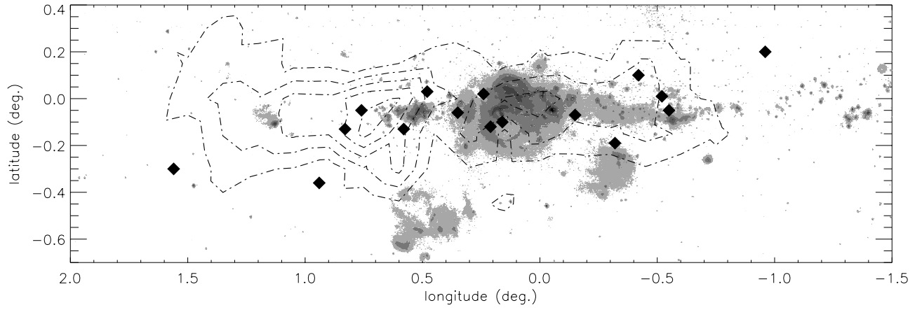
Fig. 1. Position of the observed sources (black diamonds) on the 20 \mu\text{m} image by the MSX satellite (grey levels) and the \text{C}^{18}\text{O} map by Dahmen et al. (1997, contours). M+3.06+0.34 and M+2.99-0.06 (located in the Clump 2 complex) are not shown in this figure.
