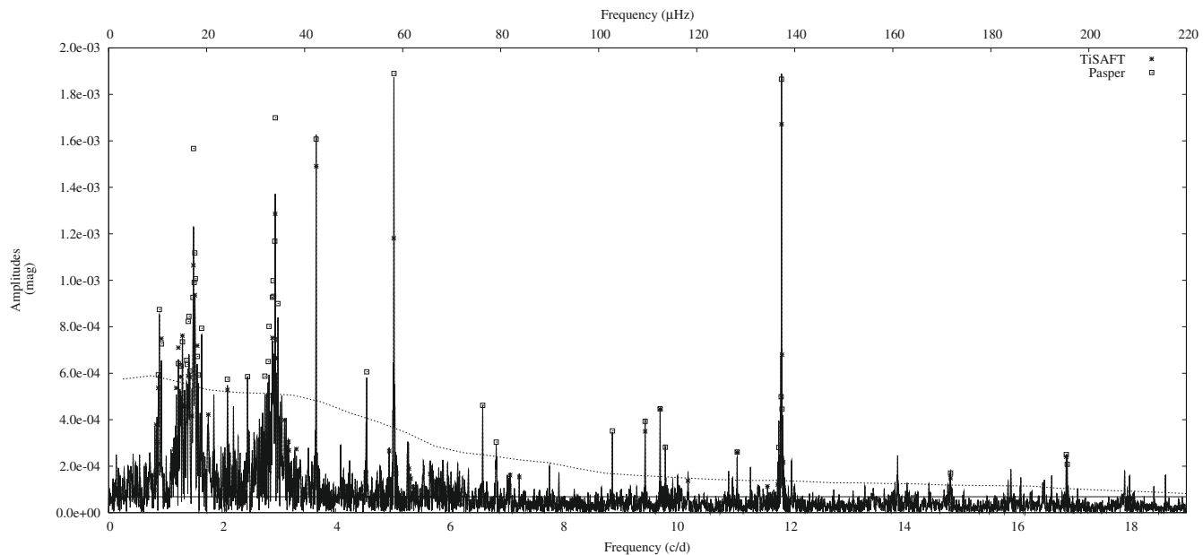
Fig. 3. Power spectrum of HD 49330 derived from the CoRoT light curve. Frequencies found by the TiSAFT and PASPER codes have been reported on the spectra. The dashed line corresponds to the limit of significance for PASPER i.e. S/N > 4 and the solid line is the limit of significance for TiSAFT with P = 99\%
