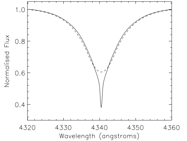
Fig. 5. Comparison of a theoretical H \gamma line with no rotational broadening (solid line) with the same line rotationally broadened by 300 \text{ km s}^{-1} (dashed line) showing that the wings of the hydrogen line are not sensitive to rotational broadening.
