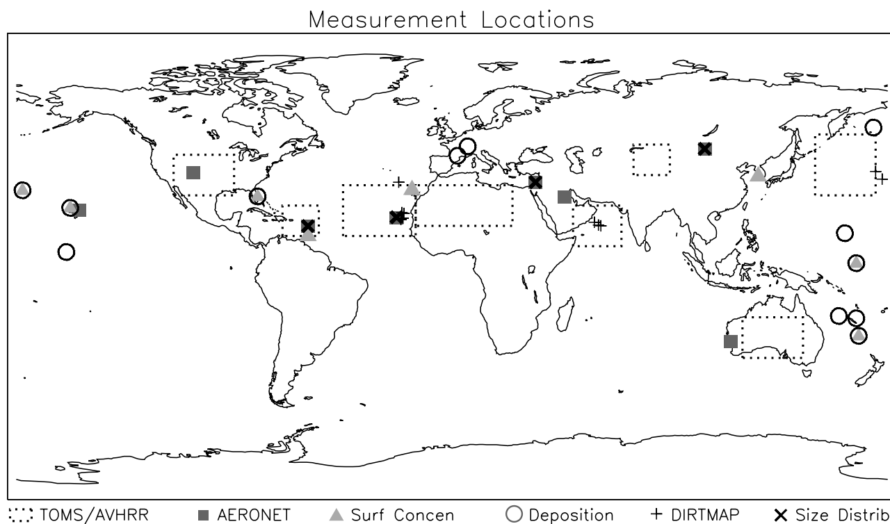
Figure 1. Locations of measurements used to evaluate the model. Satellite retrievals are averaged over the dotted regions. Squares and crosses indicate AERONET retrievals of AOT and size distribution, respectively. Triangles mark measurements of surface concentration by the University of Miami. Circles and pluses indicate measurements of deposition compiled by Ginoux et al. [2001] and DIRTMAP, respectively.
