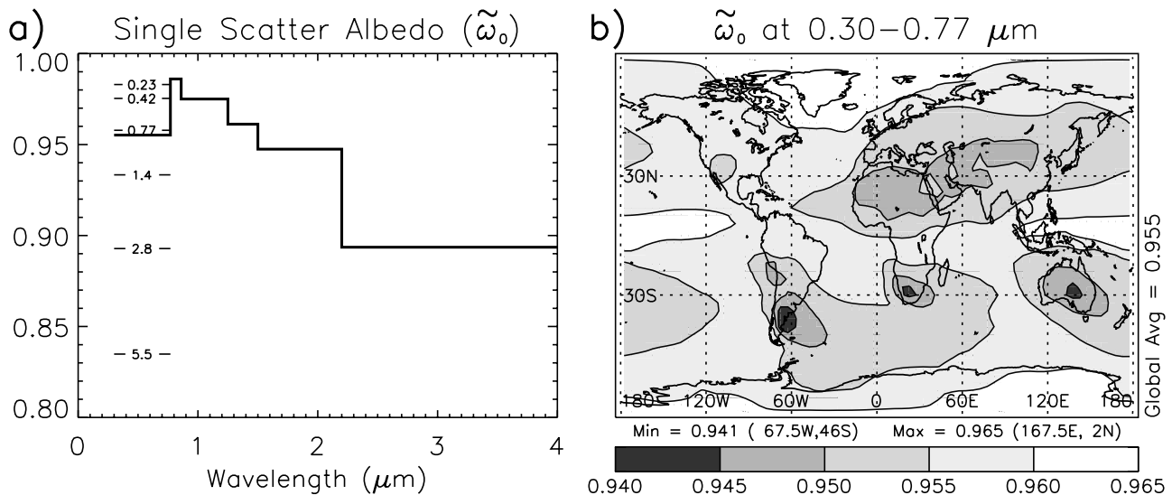
Figure 3. (a) Annual and global average of the bulk single scatter albedo \tilde{\omega}_0 , for the six spectral bands used in the calculation of solar radiative fluxes. The single scatter albedo is computed for each month as the ratio of the column scattering extinction and the column total extinction by dust. Also shown for the shortest solar band (0.30–0.77 \mu\text{m} ) is the single scatter albedo for each individual particle size category, labeled by its effective radius. (b) Geographic distribution of the annual average bulk single scatter albedo at 0.3–0.77 \mu\text{m} .
