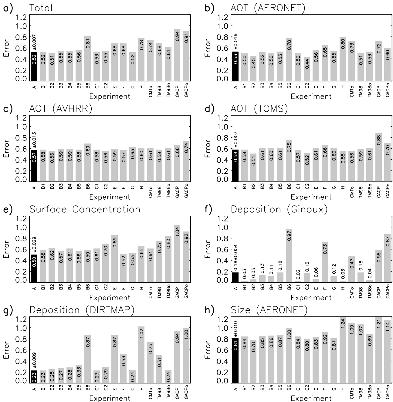
Figure 11. Total error and contribution from each data set for each sensitivity experiment described in Table 3.
