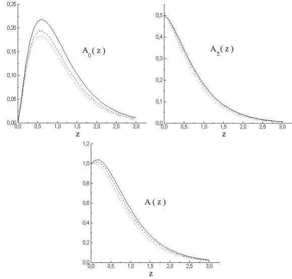
Fig. 1. Collision functions for the transition probability. Full lines: non-correlated functions A_0(z) , A_{\pm}(z) and A(z) . Dotted lines: correlated functions A_0^S(z) , A_{\pm}^S(z) and A^S(z) . Dashed lines: strongly correlated functions A_0^{SI}(z) , A_{\pm}^{SI}(z) and A^{SI}(z) for z_c = 20 .
