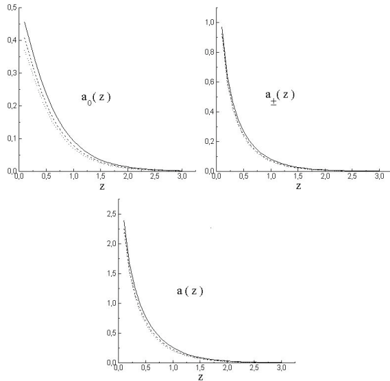
Fig. 2. Collision functions for the cross section. Full lines: non-correlated functions a_0(z) , a_{\pm}(z) and a(z) . Dotted lines: correlated functions a_0^c(z) , a_{\pm}^c(z) and a^c(z) . Dashed lines: strongly correlated functions a_0^{SI}(z) , a_{\pm}^{SI}(z) and a^{SI}(z) for z_c = 20 .
