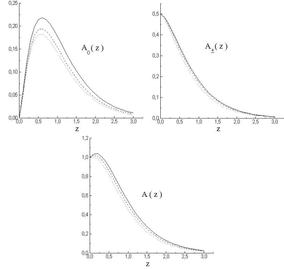
Fig. 1. Collision functions for the transition probability. Full lines: non-correlated functions A_0(z) , A_{\pm}(z) and A(z) . Dotted lines: correlated functions A_0^{\text{SI}}(z) , A_{\pm}^{\text{SI}}(z) and A^{\text{SI}}(z) for z_c = 20 .
