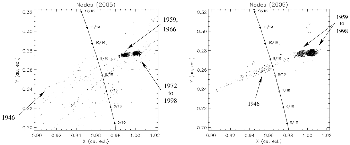
Fig. 4. Nodes of meteoroids ejected by comet 21P/Giacobini-Zinner encountering the Earth in 2005. Left: particles in the size range 0.5 to 10 mm. Right: particles in the size range 0.05 to 0.1 mm. The labels indicate the year of the perihelion return of the comet during which the particles were ejected. No visual-sized meteoroids intersect the Earth ( left ), in contrast to the smaller particles ( right ). The trail intersecting the Earth here was released during the 1946 perihelion return of the comet.
