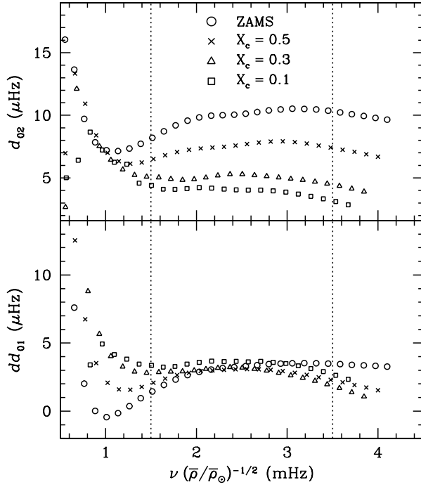
Fig. 14. The small separations d_{02} (top panel) and dd_{01} (bottom panel) are shown as functions of the scaled frequency for four 1.5 M_{\odot} models at different stages of evolution. The limits of scaled frequency used to compute the averages for the C-D diagrams are indicated by the dotted lines.
