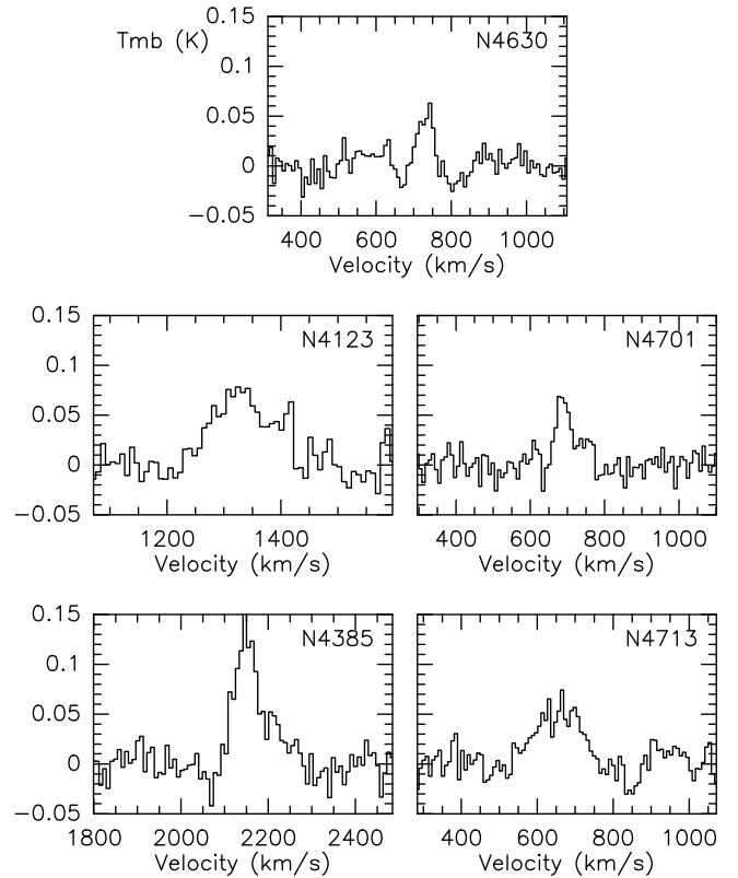
Fig. 1. CO(3–2) spectra of five galaxies detected in the observed sample. The spectra have been smoothed to 8.4 \text{ km s}^{-1} in velocity.
