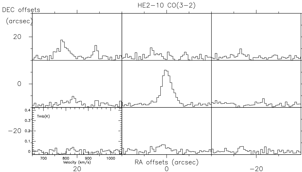
Fig. 3. CO(3–2) map of He 2–10. Nine positions spaced every 20 arcsec were observed. The spectra have been smoothed to 8.4 \text{ km s}^{-1} . Emission is detected in the center position (0, 0) at 850.6 \text{ km s}^{-1} , in the NE at (+20'', +20'') offset at 787.6 \text{ km s}^{-1} and 933.1 \text{ km s}^{-1} . These velocity components are weakly detected in 2 or 3 other positions.
