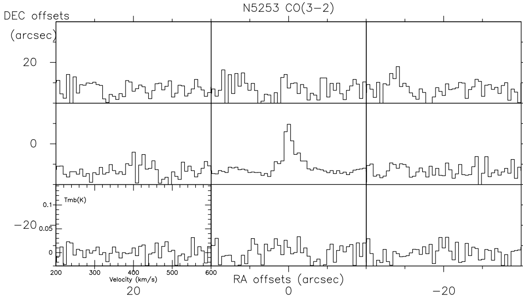
Fig. 2. CO(3–2) map of NGC 5253. Nine positions spaced every 20 arcsec were observed. The spectra have been smoothed to 8.4 \text{ km s}^{-1} . Emission is detected in the center position (0, 0) only.
