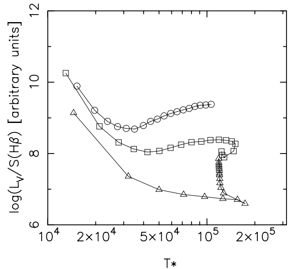
Fig. 10. The ratio L_V/S(H\beta) as a function of T_* . Same models and same presentation as in Fig. 9.
