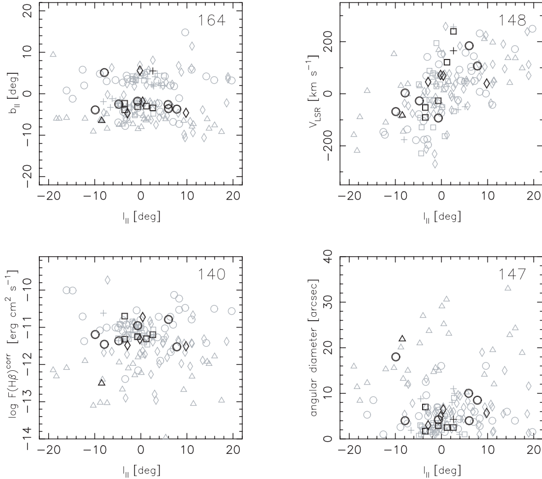
Fig. 1. Distribution in various diagrams of the PNe from our merged sample. Top left: b_{\text{II}} vs. l_{\text{II}} ; top right: V_{\text{LSR}} , the radial velocities corrected for solar motion vs. l_{\text{II}} ; bottom left: total nebular flux in \text{H}\beta corrected for reddening vs. l_{\text{II}} ; bottom right: angular diameters as a function of l_{\text{II}} . The number on the top right of each panel gives the total number of objects represented in the plot. Objects pertaining to different samples are marked by different symbols: G: circles, C: squares, B: triangles, K: plus signs, E: diamonds. (See Sect. 2.2 for detailed definitions.) Symbols for [WR] PNe are thicker than for the rest of PNe.
