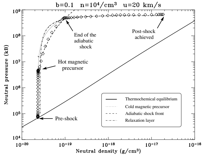
Fig. 2. Steady state analytic relations between pressure and mass density are compared to an overlaid future C-shock (diamonds). The parameters of the shock are u = 20 \text{ km s}^{-1} , n = 10^4 \text{ cm}^{-3} and b = 0.1 , time is t = 10^2 \text{ yr} . The additional necessary parameters B_p and \dot{E}_p are read in the shock model at the end of the precursor (they are not fitted).
