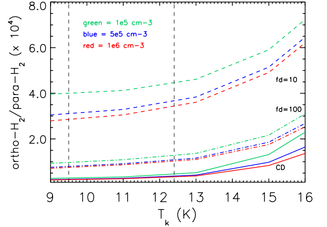
Fig. 7. Variation of the ortho-to-para H 2 ratio as a function of the kinetic temperature, for densities of 1 \times 10^5 (green), 5 \times 10^5 (blue) and 1 \times 10^6 (red) cm -3 . Three depletion factors at steady-state are presented: complete depletion (CD: solid lines), depletion factor =100 (dot-dashed lines) and depletion factor =10 (dashed lines). The thin dashed vertical lines present the [9.5–12.4] K range.
