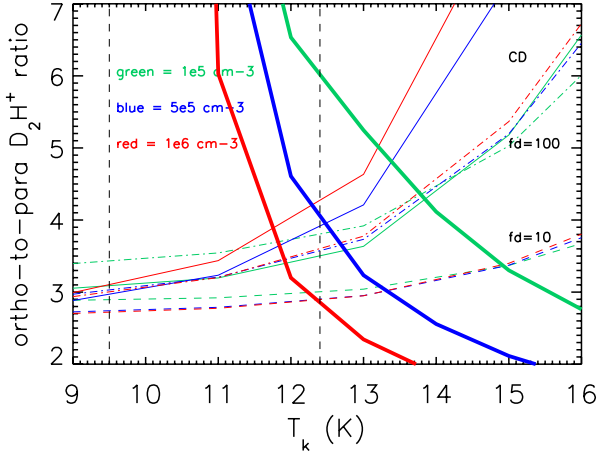
Fig. 5. Variation of the ortho-to-para D 2 H + ratio as a function of the gas temperature, for densities of 1 \times 10^5 (green), 5 \times 10^5 (blue) and 1 \times 10^6 (red) cm -3 . The thick lines show the ratio derived from observations, using non-LTE modeling, and can be considered as upper limits, whereas the thin lines show the chemical model results. Three depletion factors at steady-state are presented: complete depletion (CD: solid lines), depletion factor =100 (dot-dashed lines) and depletion factor =10 (dashed lines). The thin dashed vertical lines present the [9.5–12.4] K range.
