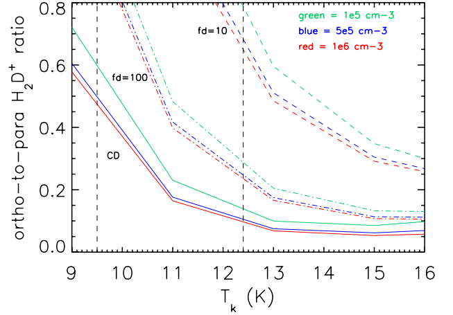
Fig. 6. Prediction of the ortho-to-para H 2 D + ratio as a function of the gas temperature, for densities of 1 \times 10^5 (green), 5 \times 10^5 (blue) and 1 \times 10^6 (red) cm -3 . Three depletion factors at steady-state are presented: complete depletion (CD: solid lines), depletion factor =100 (dot-dashed lines) and depletion factor =10 (dashed lines). The thin dashed vertical lines present the [9.5–12.4] K range.
