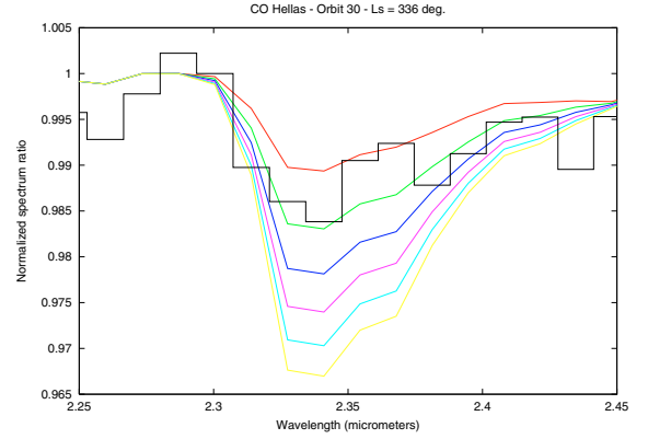
Fig. 7. Black curve: the averaged observed spectrum over Hellas for Ls = 335.7 deg (orbit 30-1) divided by the reference spectrum taken at the summit of Olympus Mons. Color curves: synthetic ratio of spectra, calculated for the surface pressure and the airmass of the observation, with, from top to bottom : CO = 500, 1000, 1500, 2000, 2500 and 3000 ppm.
