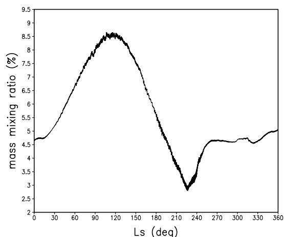
Fig. 2. Evolution of the mixing ratio of non-condensable species over the Hellas basin (35S, 65E) as a function of the solar longitude L_s . A doubling of the mixing ratio is expected at L_s = 90\text{--}150 deg with respect to its value at L_s = 270\text{--}10 deg.
