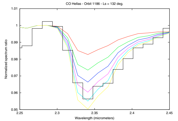
Fig. 8. Black curve: the averaged observed spectrum over Hellas for Ls = 132.0 deg (orbit 1186-4) divided by the reference spectrum. Models: see Fig. 7.
