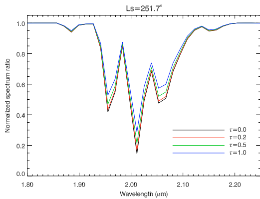
Fig. 6. Effect of dust scattering on the depth of the CO 2 band at 2.0 \mu\text{m} . The surface pressure is 10 mbars. Dust opacity, from top to bottom : 1.0, 0.5, 0.2, 0.0.
