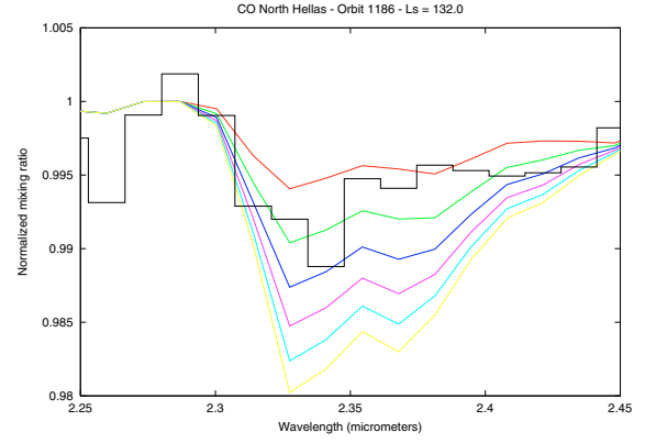
Fig. 12. Black curve: the averaged observed spectrum at the north of Hellas (lat. 23S) for L_s = 132.0 deg (orbit 1186-4) divided by the reference spectrum. Models: see Fig. 7.
