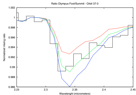
Fig. 3. Black curve: ratio of two averaged OMEGA spectra, recorded at the foot and at the summit of Olympus Mons respectively (Orbit 37-3), in the region of the CO 2.35\text{ }\mu\text{m} band. The summit spectrum, corresponding to the summation of 352 individual spectra, is taken as a reference. Color curves: synthetic ratios of spectra, using a radiative transfer code without scattering ( P_s = 1.1\text{ mbar} at the summit, 6.5\text{ mbar} at the foot). From top to bottom; CO = 500, 1000 and 1500 ppm. The best fit corresponds to CO = 1000 \pm 400 ppm ( \pm \sigma ). Including a correction to account for scattering effects (see text), the result becomes CO = 1100 \pm 500 ppm.
