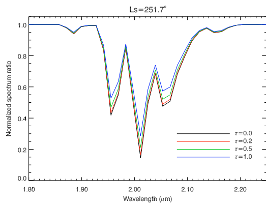
Fig. 6. Effect of dust scattering on the depth of the \text{CO}_2 band at 2.0 \mu\text{m} . The surface pressure is 10 mbars. Dust opacity, from top to bottom : 1.0, 0.5, 0.2, 0.0.
