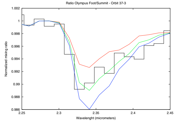
Fig. 3. Black curve: ratio of two averaged OMEGA spectra, recorded at the foot and at the summit of Olympus Mons respectively (Orbit 37-3), in the region of the CO 2.35\ \mu\text{m} band. The summit spectrum, corresponding to the summation of 352 individual spectra, is taken as a reference. Color curves: synthetic ratios of spectra, using a radiative transfer code without scattering ( P_s = 1.1\ \text{mbar} at the summit, 6.5\ \text{mbar} at the foot). From top to bottom; CO = 500, 1000 and 1500 ppm. The best fit corresponds to CO = 1000 \pm 400\ \text{ppm} ( \pm \sigma ). Including a correction to account for scattering effects (see text), the result becomes CO = 1100 \pm 500\ \text{ppm} .
