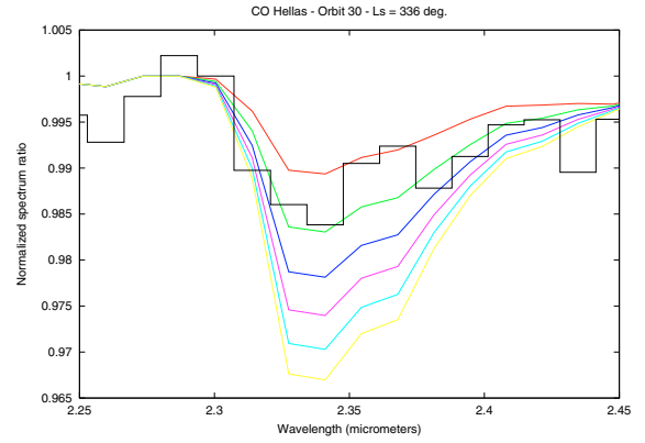
Fig. 7. Black curve: the averaged observed spectrum over Hellas for L_s = 335.7 \text{ deg} (orbit 30-1) divided by the reference spectrum taken at the summit of Olympus Mons. Color curves: synthetic ratio of spectra, calculated for the surface pressure and the airmass of the observation, with, from top to bottom : CO = 500, 1000, 1500, 2000, 2500 and 3000 ppm.
