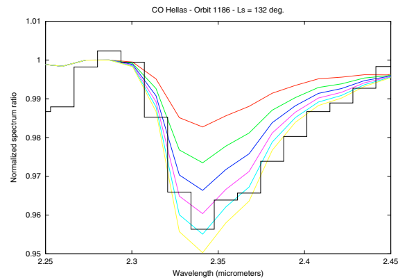
Fig. 8. Black curve: the averaged observed spectrum over Hellas for L_s = 132.0 \text{ deg} (orbit 1186-4) divided by the reference spectrum. Models: see Fig. 7.
