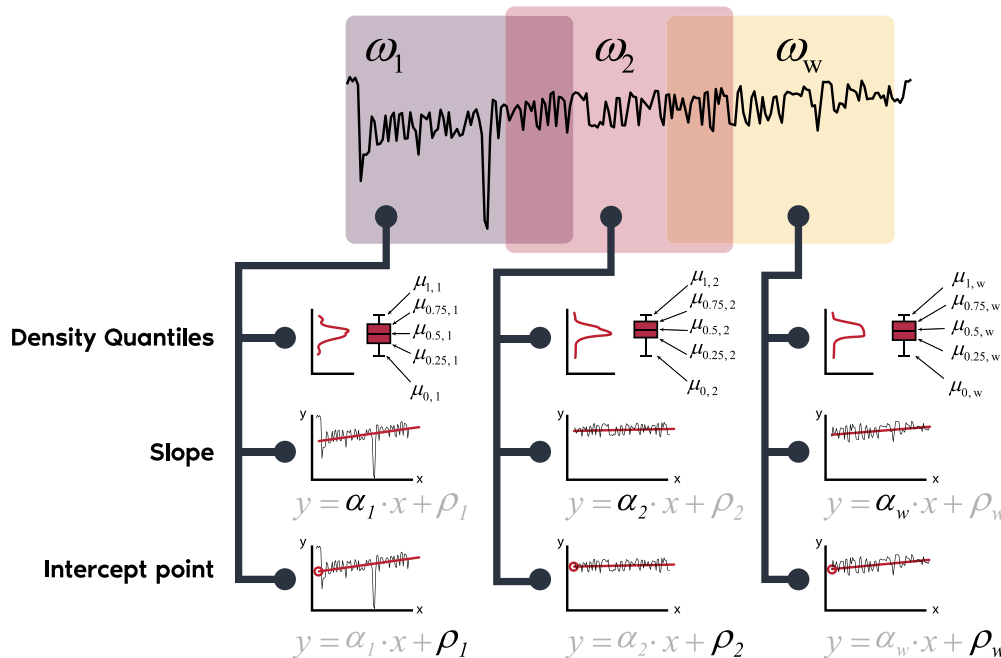
Fig. 4. Example of feature extraction through sliding windows.
