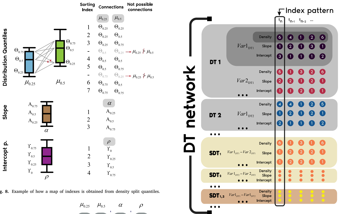
Fig. 10. Example of a DT network.
