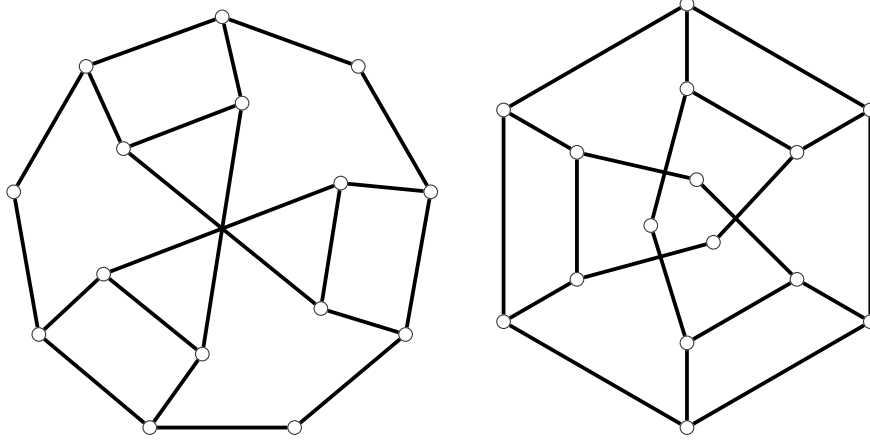
Figure 2: A symmetric graph of order 15 and odd-girth 7 which do not map to C_5 .
