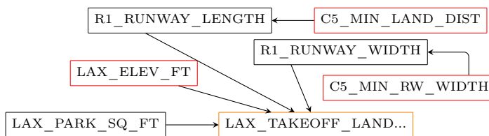
Figure 1: Example of a SIM and a SIG. Partial reproduction of Fig.1 in [LRB20].
