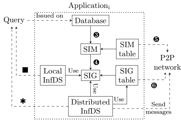
(b) Architecture of an application in the network.
