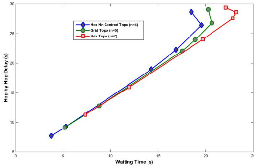
Fig. 14. Correlation between The hop-by-hop delay and the average waiting time.
