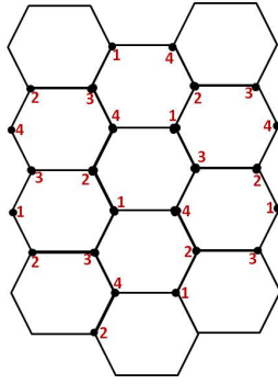
Fig. 10. Non-centered hexagonal topology.
