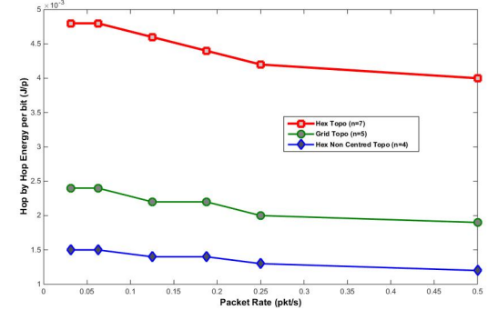
Fig. 16. Average consumed energy per useful bit.
