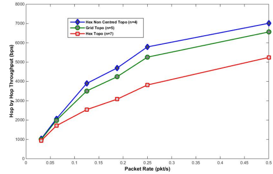
Fig. 15. Average Hop-by-hop Throughput.
