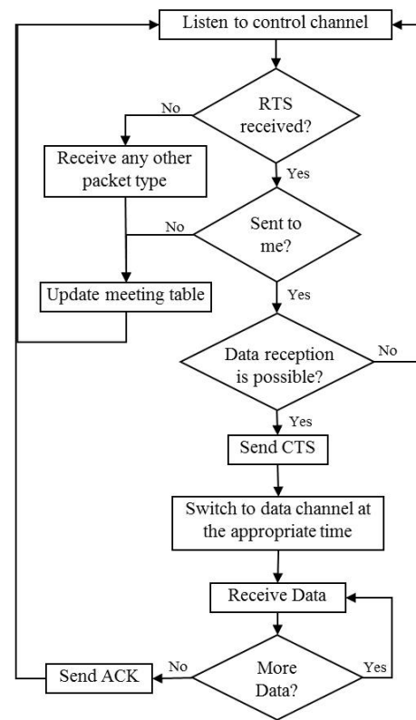
Fig. 6. Flowchart of the receiver behavior.
