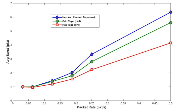
Fig. 12. Average Burst size.
