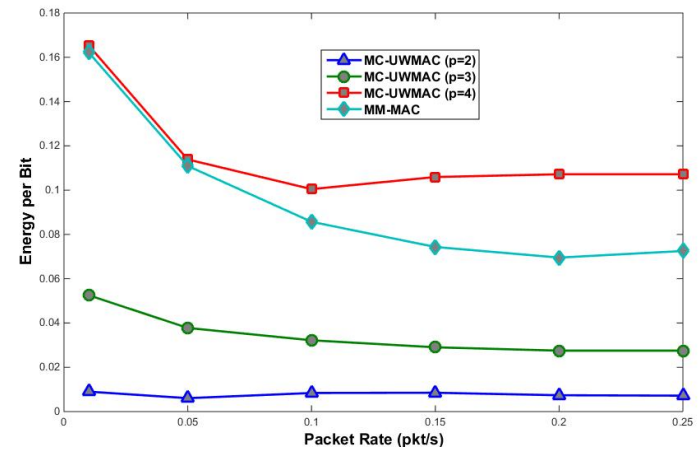
Fig. 20. Energy consumption per bit.
