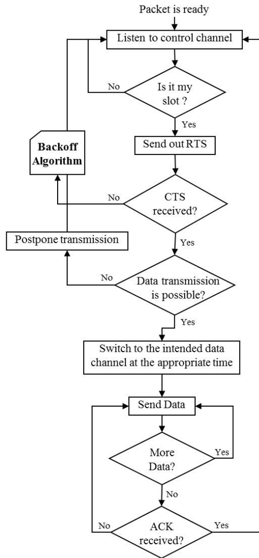
Fig. 5. Flowchart of the sender behavior.
