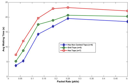
Fig. 13. Average waiting time (queuing time).
