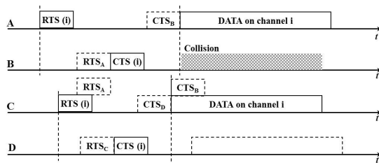
Fig. 1. Long-Delay Hidden Terminal Problem.
