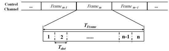
Fig. 2. MC-UWMAC frame structure.
