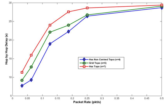
Fig. 11. Average Hop-by-hop delay.
