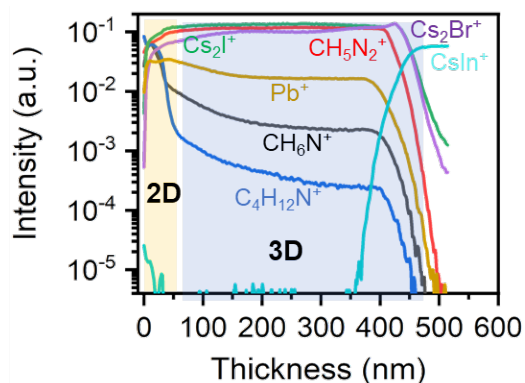
Figure S10. ToF-SIMS depth profile of the 3D/PP-2D (BA 2 MA 2 Pb 3 I 10 ) HaP stack deposited on top of ITO shows the distribution of different ions across the thickness and the sharpness of the heterointerface.
