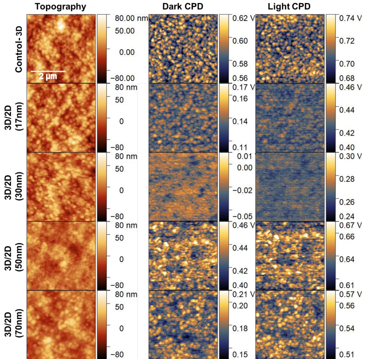
Figure S31. Representative images showing the AFM topography, and contact potential difference (CPD) in the dark and under illumination (590 nm, \sim 2.4 mW/cm 2 ) for different 2D thicknesses.
