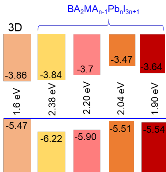
Figure S15. Plot showing predicted values of band energy levels of 2D, BA_2MA_{n-1}Pb_nI_{3n+1} perovskites with different n-values (n=1-4), calculated using single-point calculations with GGA-PBE functional combined with DFT-1/2, including spin-orbit coupling.
