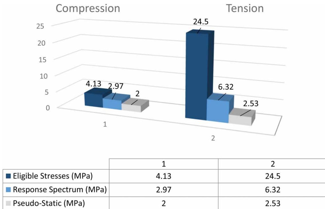
Figure 13 | Calculated stress values compared to eligible stresses.
