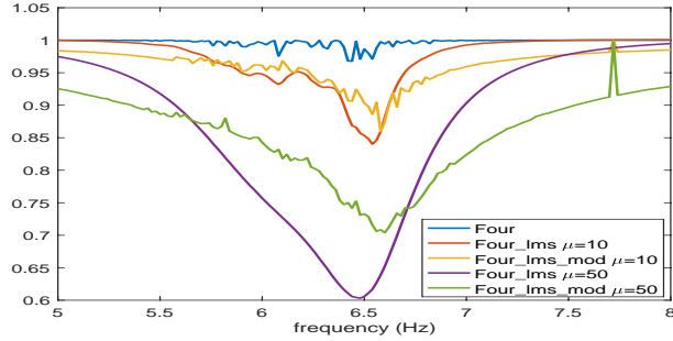
Figure 2. Comparison of spectral decompositions for multiple components model for the highest DF among the BSPM leads.
