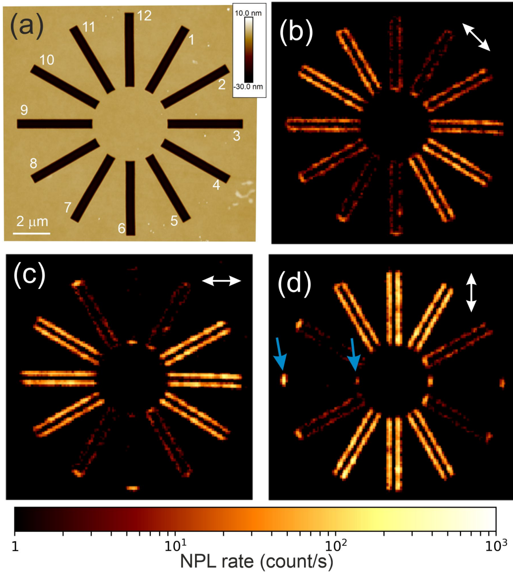
Figure 5: (a) Atomic force image displaying the circularly symmetric pattern fully etched in the ITO. Corresponding NPL maps taken with an incident polarization angle of 45^\circ (b), 0^\circ (c) and 90^\circ (d) (white double arrows). The blue arrows mark the effect of the ion beam milling strategy (see text for details). The intensity is in logarithmic scale to help visualizing even the dimmest regions.
