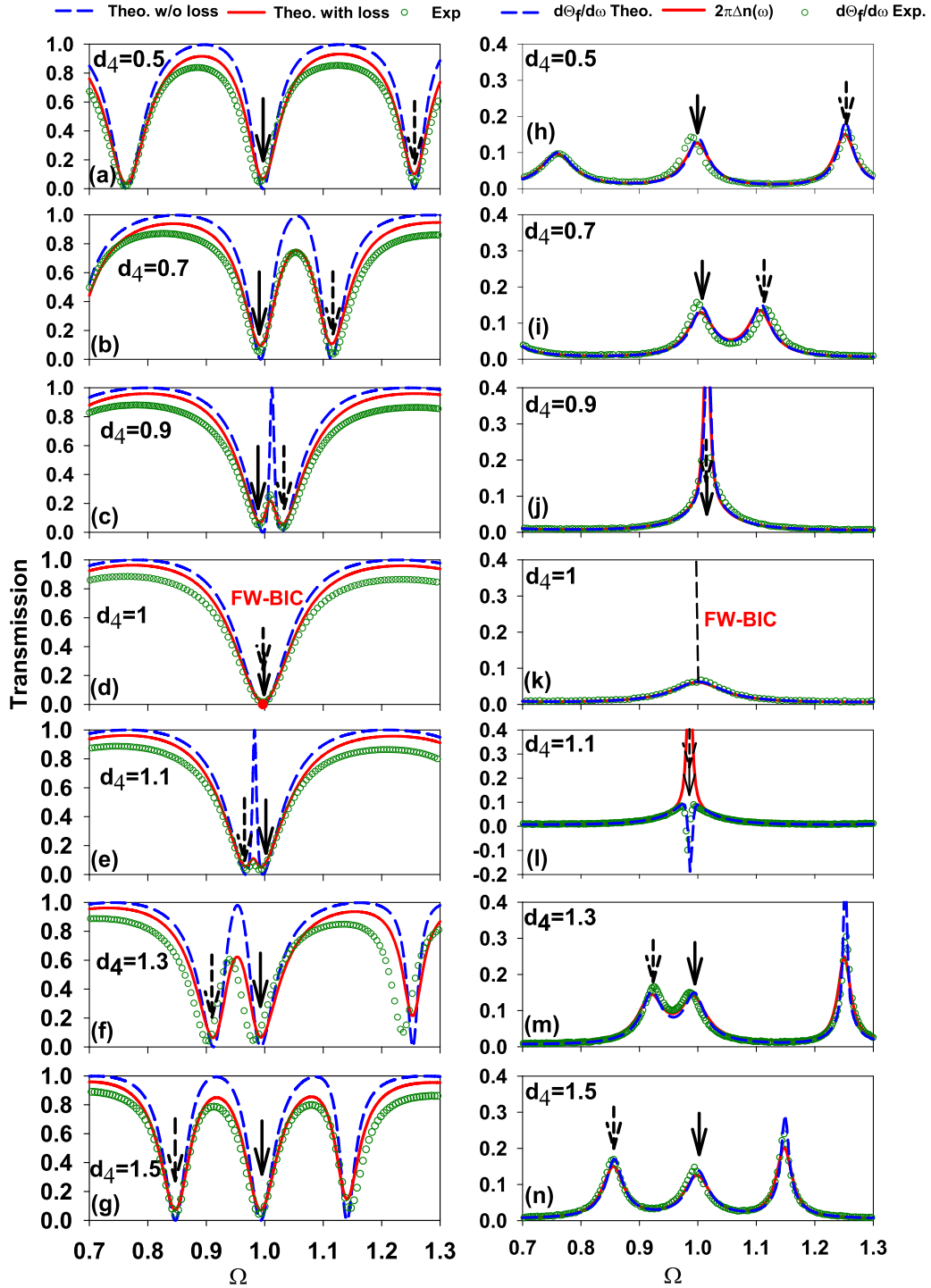
FIG. 7. (a)–(g) (Left panel) Transmission coefficient versus \Omega for different values of d_4 around d_4 = 1 . The lengths of the arms of the loop are taken such that d_2 = 0.2 and d_3 = 1.8 . Blue and red curves correspond to theoretical results without and with loss, respectively, whereas green curves correspond to experimental results. (h)–(n) (Right panel) Variation of the DOS \Delta n(\omega) (red lines) and the derivative of the Friedel phase \frac{d\theta_f}{d\omega} (blue dashed curves) for different values of d_4 . The theoretical results of \frac{d\theta_f}{d\omega} (blue dashed lines) are validated by the experimental data (green open circles). The position of FW BIC is indicated by the filled circle in (d) and by dashed line in (k). The solid and dashed arrows indicate the positions of transmission dips associated to the two interacting modes of the DBCS.
