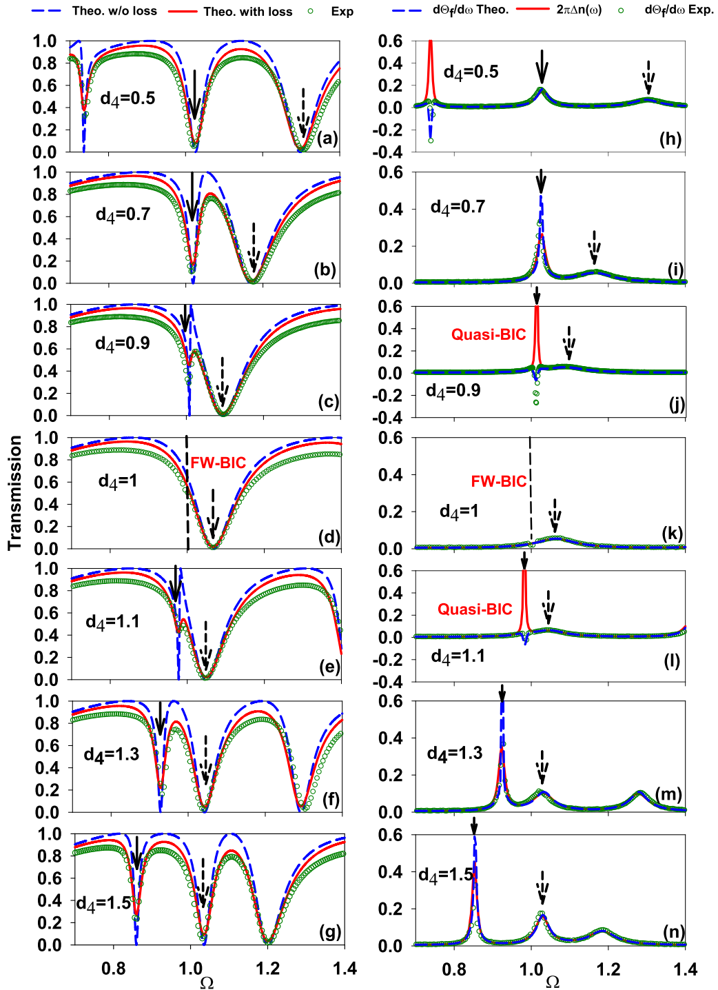
FIG. 3. (a)–(g) (Left panel) Transmission coefficient versus \Omega for different values of d_4 around d_4 = 1 for d_1 = 0.3 . The lengths of the arms of the loop are taken such that d_2 = 0.2 and d_3 = 1.8 . Blue and red curves correspond to theoretical results without and with loss, respectively, whereas green curves correspond to experimental results. (h)–(n) (Right panel) Variation of the DOS (red lines) and the derivative of the Friedel phase \frac{d\theta_f}{d\omega} (blue dashed curves) for different values of d_4 . The position of FW BIC is indicated by the dashed lines in (d) and (k). The theoretical results of \frac{d\theta_f}{d\omega} (blue dashed lines) are validated by the experimental data (green open circles). The solid and dashed arrows indicate the positions of the transmission dips.
