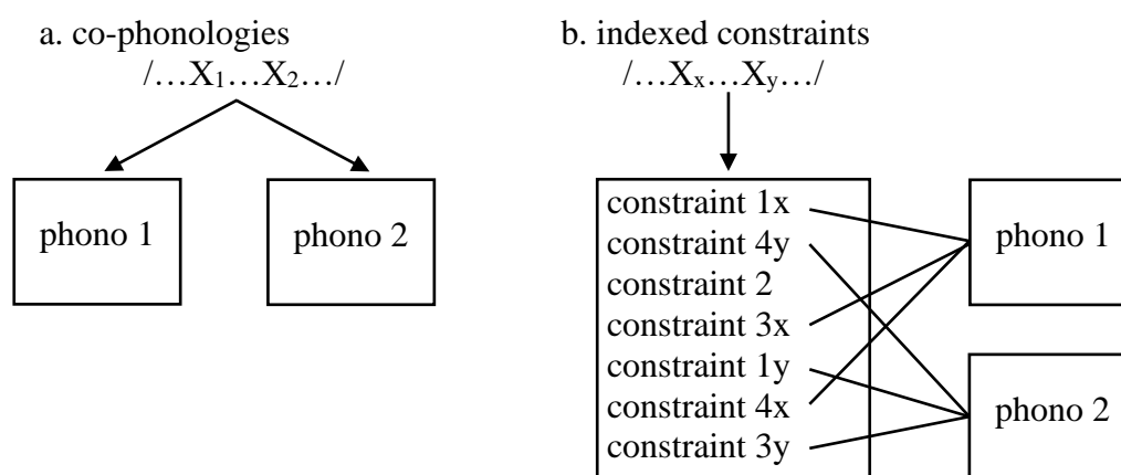
Figure 8: Representations of co-phonologies and indexed constraints
