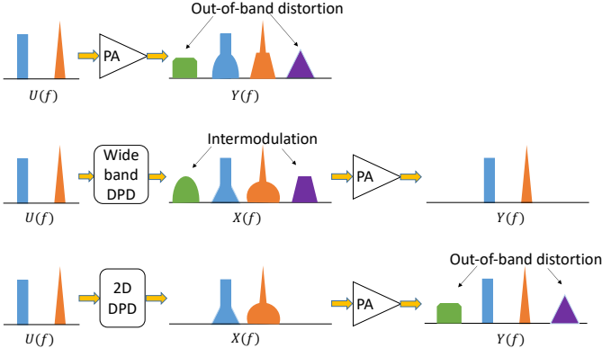
Fig. 1. Spectral expansion by PA and DPD for dual-band signal.
