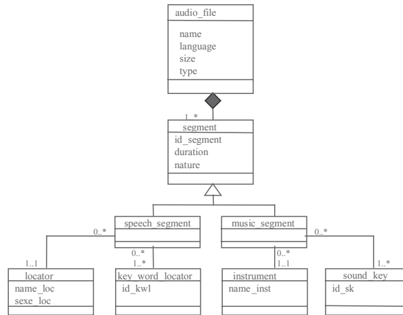
Fig. 3. Audio model
