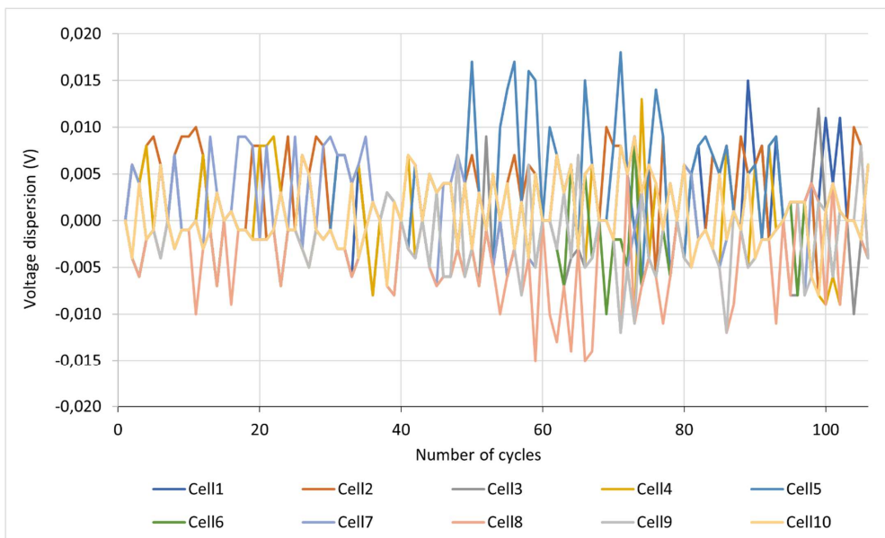
Figure 8. Voltage dispersion per cell (battery 5).
