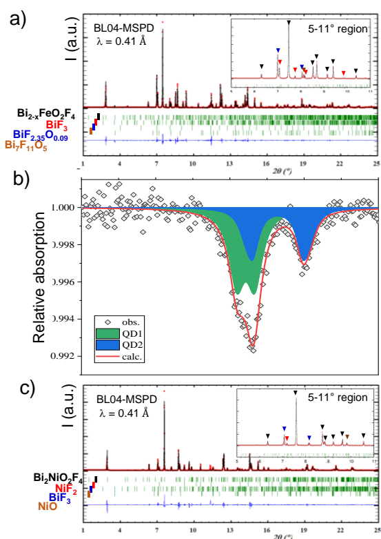
Figure 3: a) BiFeOF SXPDP Rietveld refinement with detail of the side-phases. The arrows in the inset are associated by color to the phases reported at the bottom. b) BiFeOF ^{57}\text{Fe} Mössbauer spectrum at 293 K fitted with QD1 and QD2 components and their sum (red line). c) BiNiOF Rietveld refinement of the synchrotron data.
