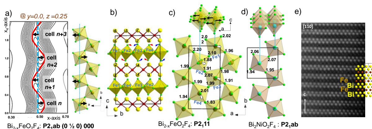
Figure 2 : a) \text{BiFeOF} : 4D approach : (x, x4) Fourier section around the Fe position (summed 1 Å in y and z ). The red line corresponds to the refined displacive wave around the central position (blue line) with the corresponding structural model (right). b) Projected structure in the (b, c) plane with evidences of the octahedral tilt around the c -axis. c) Projected perovskite slab in the (b, c) plane with main Fe sheets along the a -axis (black arrows) and ferroelectric displacements in the \text{FeF}_6 octahedra (white arrows). d) \text{BiFeOF} [110] HAADF STEM image where the contrast is proportional to z^2 , i.e. heavy atoms are brighter. e) \text{BiNiOF} perovskite slab
