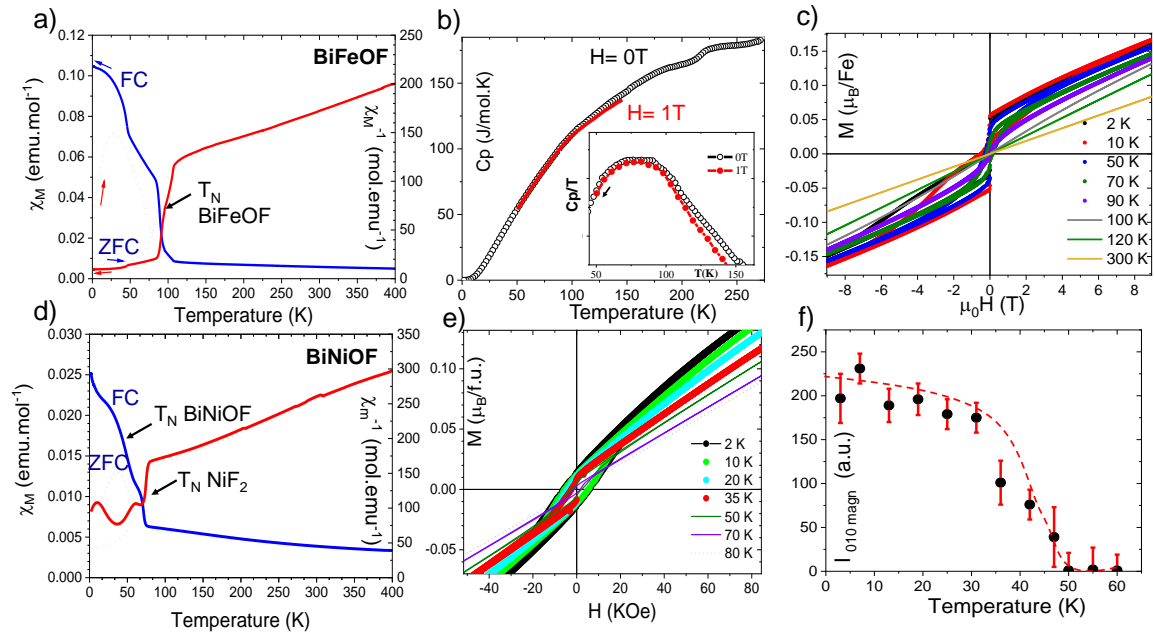
Figure 5 : BiFeOF : a) \chi(T) and \chi^{-1}(T) at H=0.1 T. b) C_p(T) at 0T and 1T. c) M(H) at various temperatures. BiNiOF : d) \chi(T) and \chi^{-1}(T) at H=0.5 T. e) M(H) at various temperatures with weak ferrimagnetism. f) Intensity of the 010 magnetic contribution.
