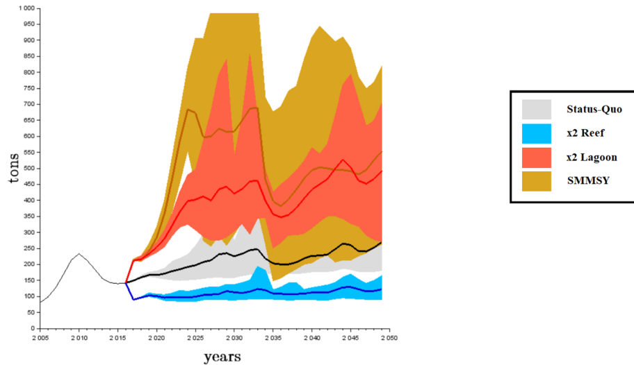
Fig. 9 a Catches per fleets trajectories: The 100 simulated trajectories are represented by the coloured areas depending on the management strategy. The solid lines display the average of these 100 trajectories. The four first fleets (up) operate on the lagoon and the three other ones (down) operate on the fore reef (with “no boat” it is impossible
