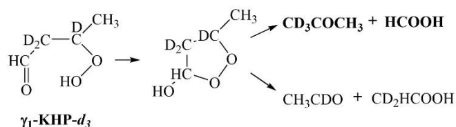
Scheme 1. Decomposition of 3-hydroperoxybutanal- d_3 ( \gamma -KHP- d_3 ) into carbonyl + acid pairs via the Korcek mechanism. 3-hydroperoxybutanal- d_3 is the main KHP observed in n -butane- d_4 oxidation. The Korcek pathway observed in this study is indicated in bold.
