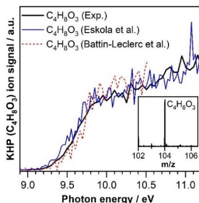
Figure 1. Photoionization spectrum of KHP ( C_4H_8O_3 ), identified as 3-hydroperoxybutanal,[9] measured at \sim 590 K, 740 Torr and compared with spectra from Eskola et al.[9] and Battin-Leclerc et al.[8] The insert represents the typical C_4H_8O_3 mass signal recorded at a photon energy of 10.5 eV.
